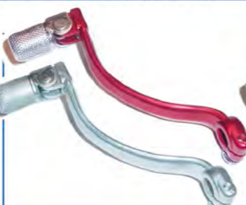
Ref. 009059 • 24700KZ4-J50 PALANCA CAMBIO GEAR LEVER Honda CR 125 2 T (2001-03)
